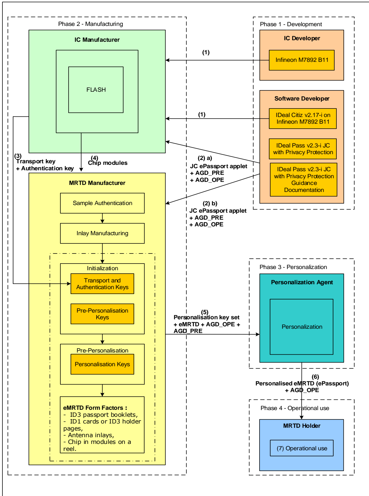
Figure 2: TOE life-cycle
